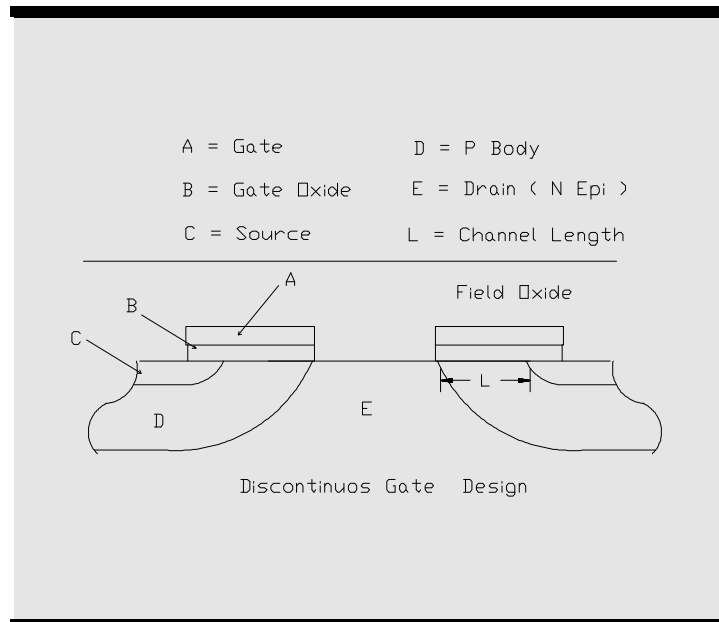
Fig 1. Cross Section of Vertical DMOS transistor
