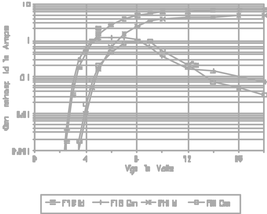
Fig 4. Gm vs Id Polyfet and PHI F1B equivalent die
