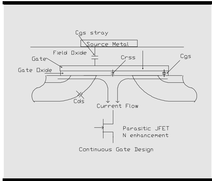
Fig 2. VDMOS Continuous Gate Design
