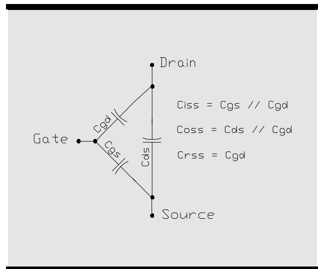
Fig 5 DMOS Capacitances
