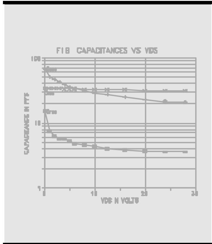
Fig 6. Capacitance vs V_{ds} for Polyfet F1B devices
