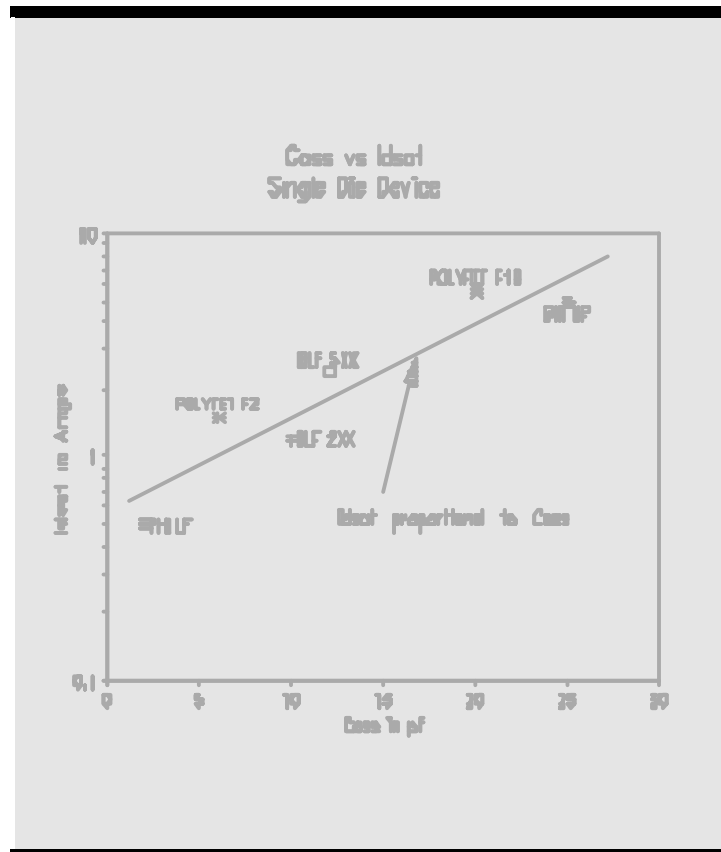
Fig 8. Id vs Coss for a single die device
