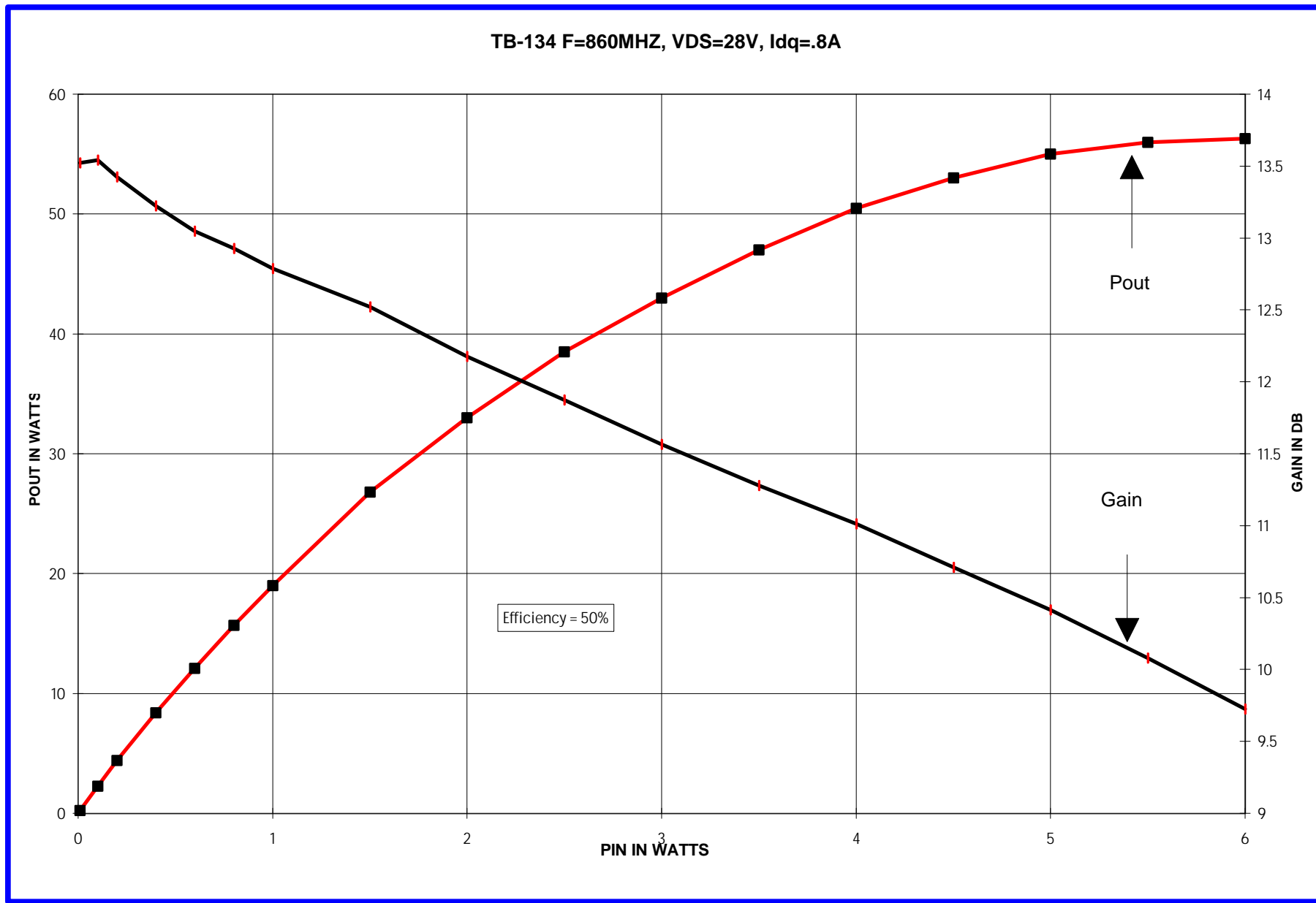
Pin vs Pout W Chart 1
