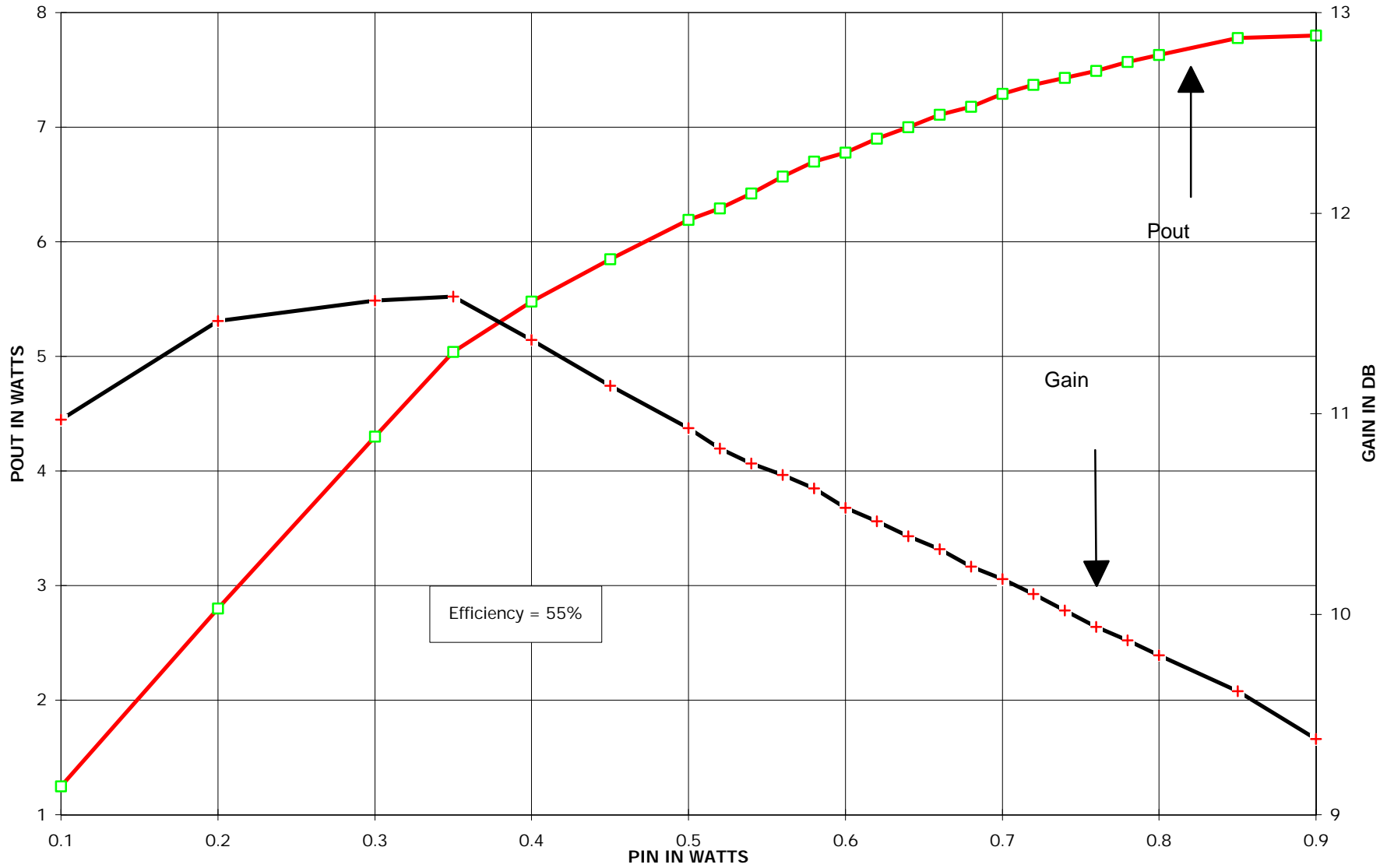
L2711 Pin vs Pout F=500 MHZ; Idq=.4; Vds=7.5V
