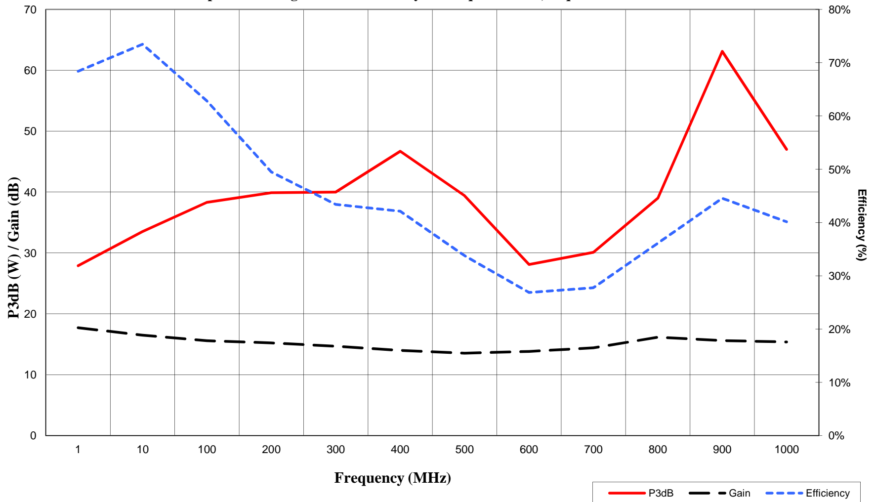
P3dB power/P3dB gain/P3dB efficiency vs Freq: Vds=48V, Idq=0.3A
